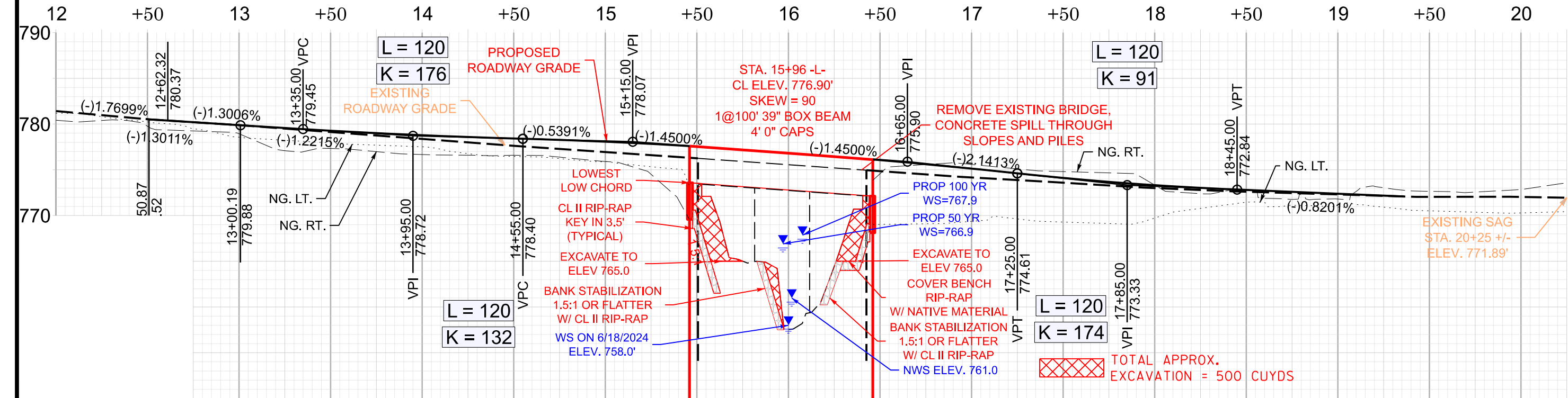
PROFILE ALONG BRIDGE
